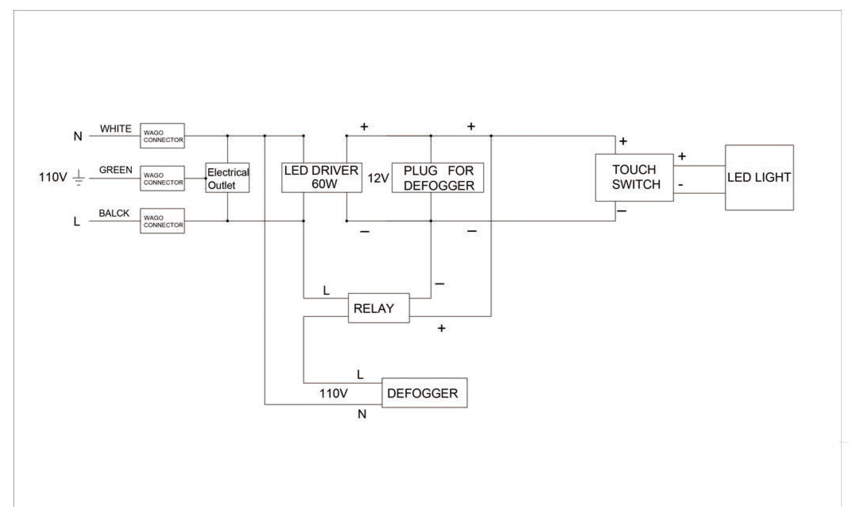
Circuit Diagram
