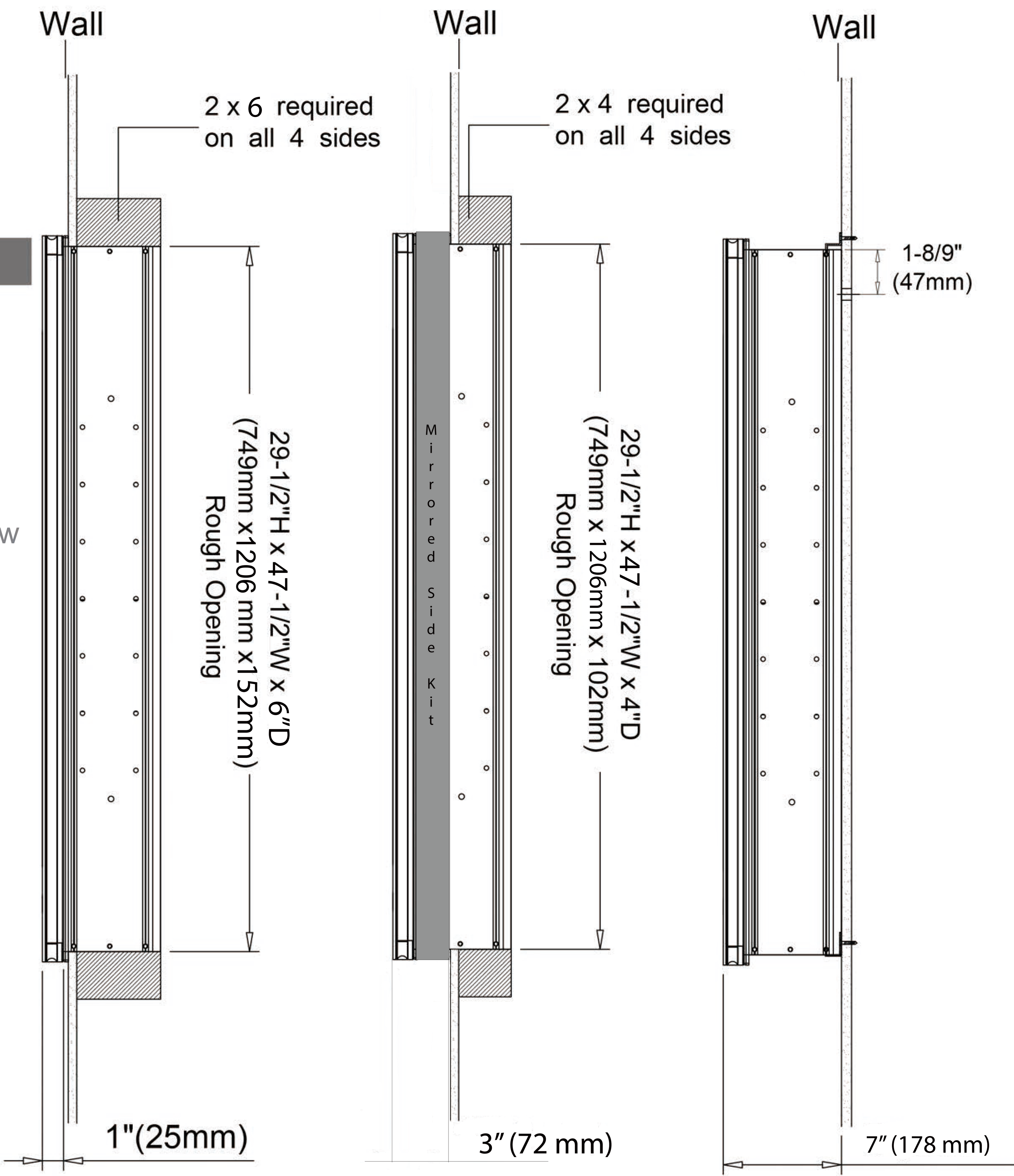
Recessed Mount
