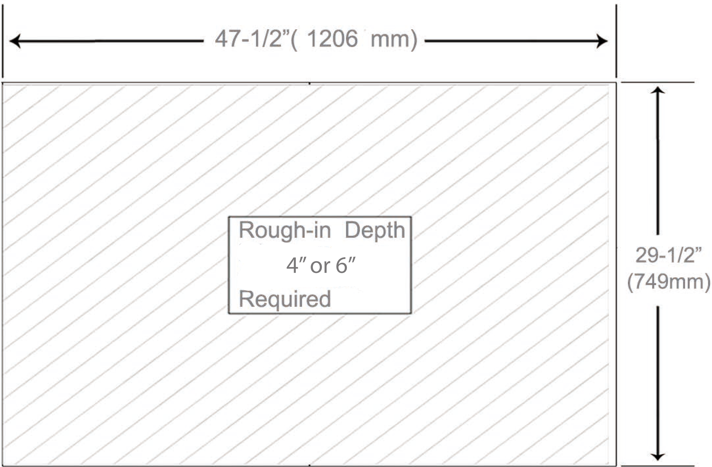
Rough-in Dimensions
