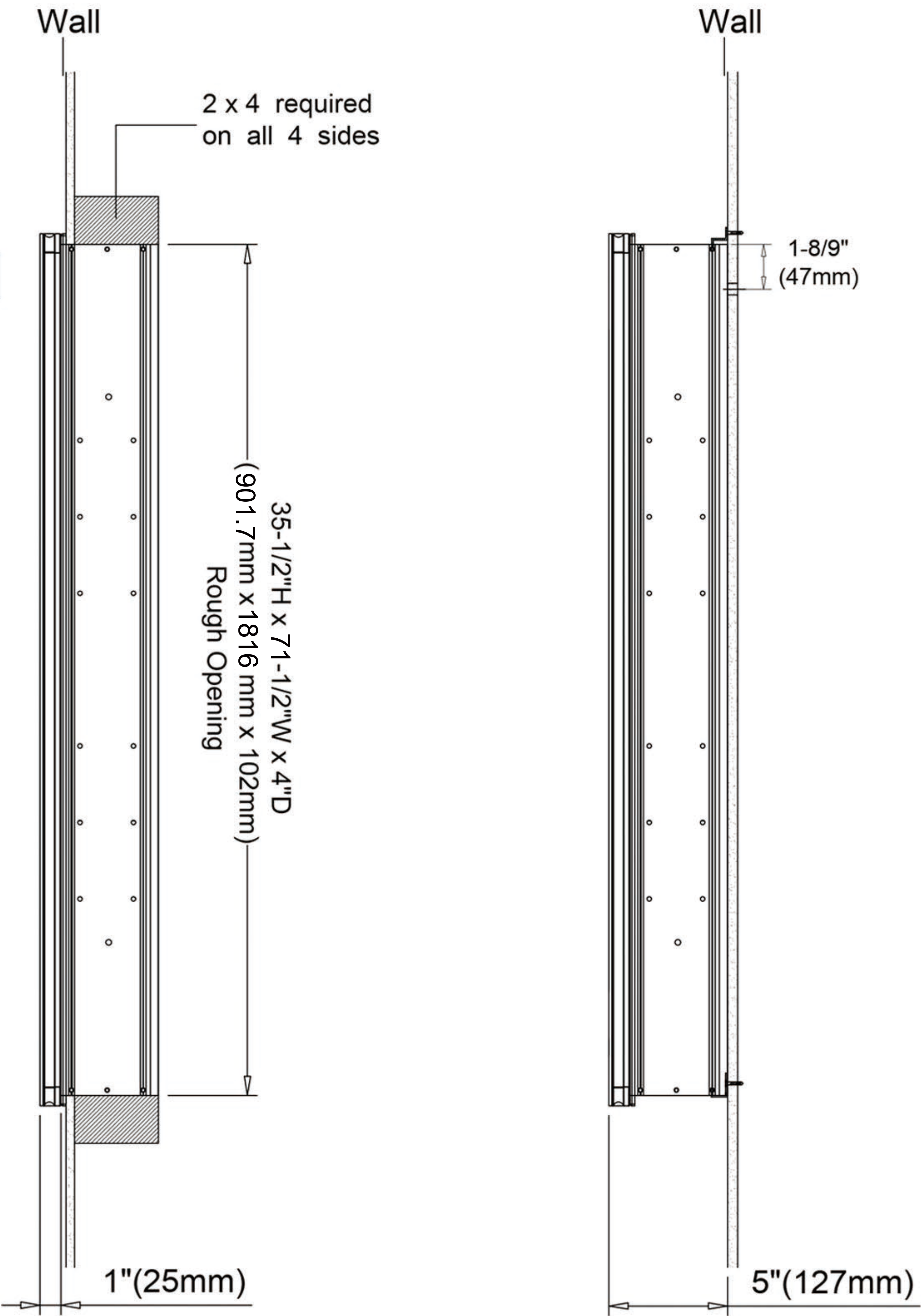
Recessed Mount
