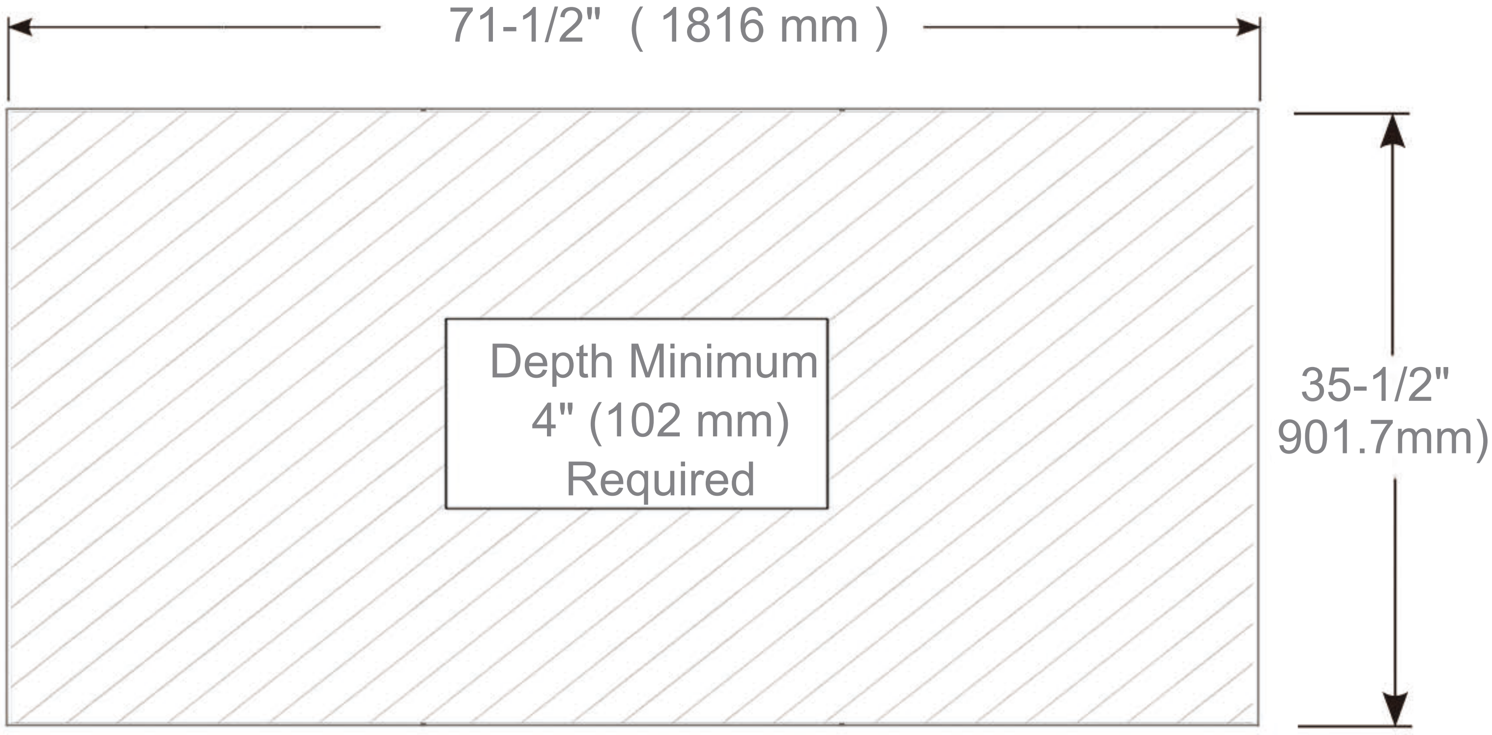
Rough-in Dimensions
