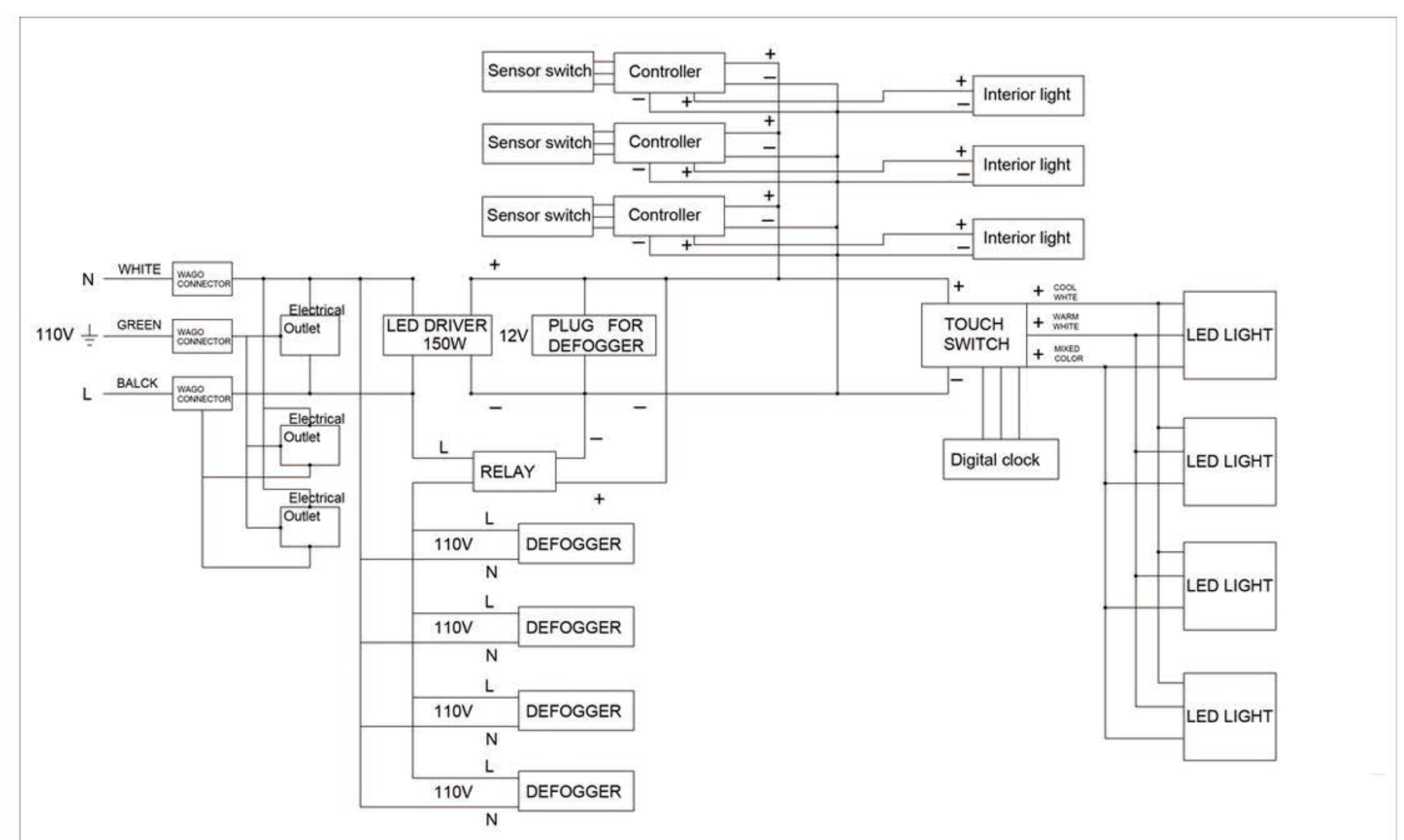
Circuit Diagram
