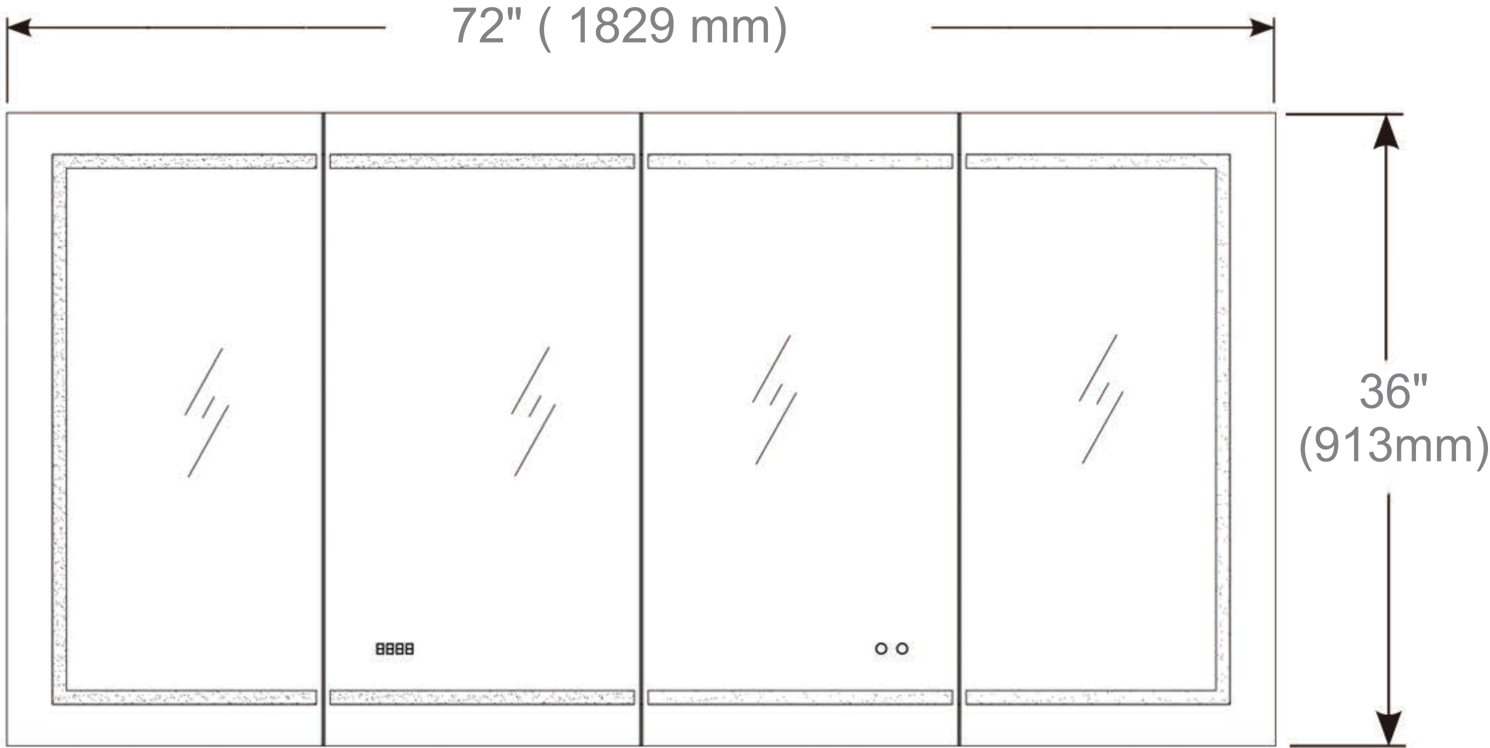
Cabinet Dimensions
